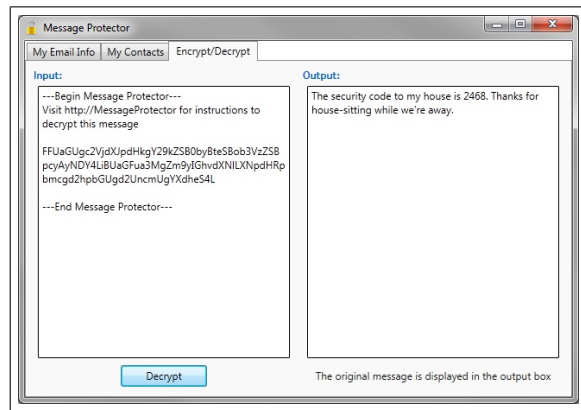
Figure 3.4: Message decryption
