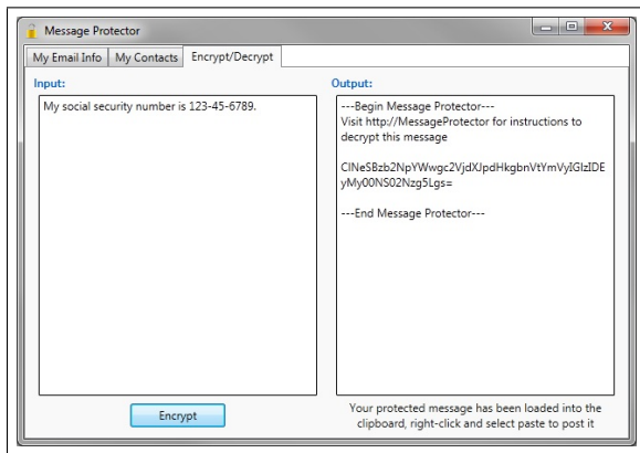
Figure 3.3: Message encryption
